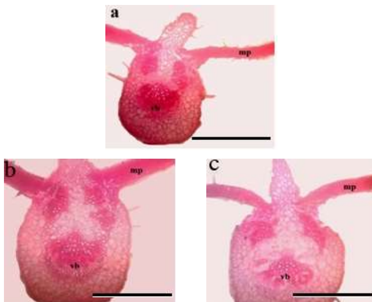
Figure 1. Leaf anatomy a. Control (seed soaking and foliar spray with tap water), b. SA seed soaking + MLE foliar spray, and c. MLE seed soaking + SA foliar spray. (mp = mesophyll and vb= vascular bundle). Scale bar = 200 \mu
